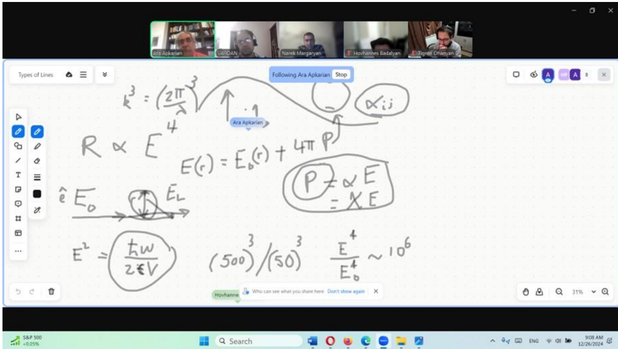
Ara Apkarian's physics equations that explain confined light mechanisms
